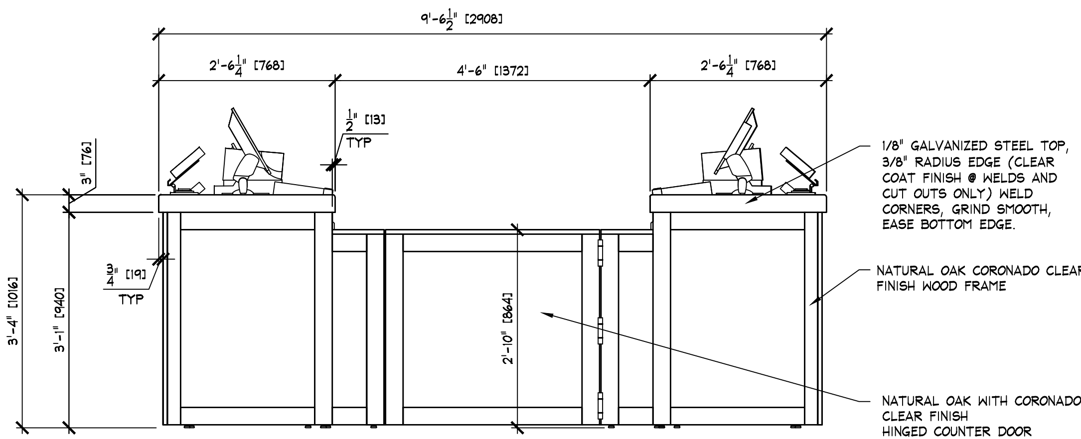
EXTERIOR ELEVATION
