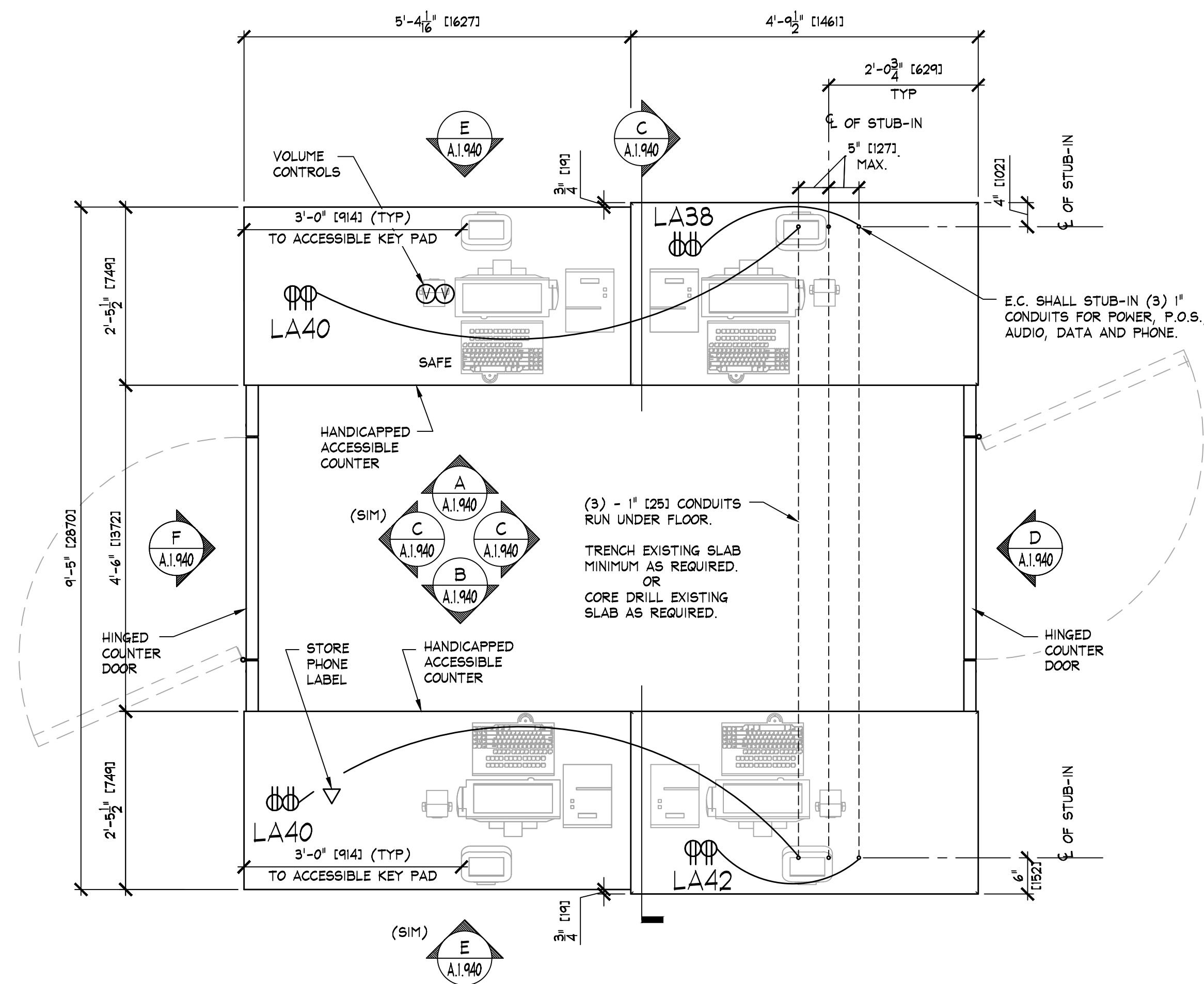
PLAN VIEW ISLAND COUNTER
