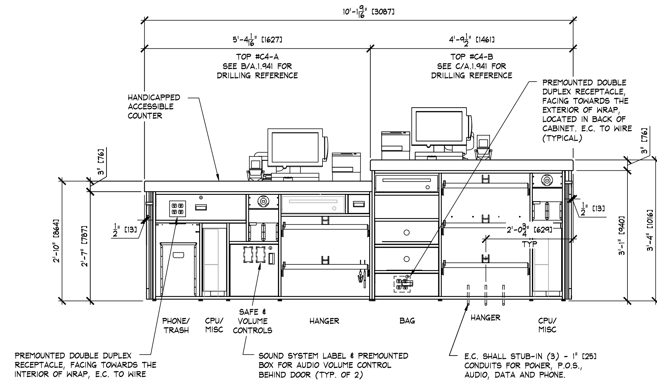
INTERIOR ELEVATION
