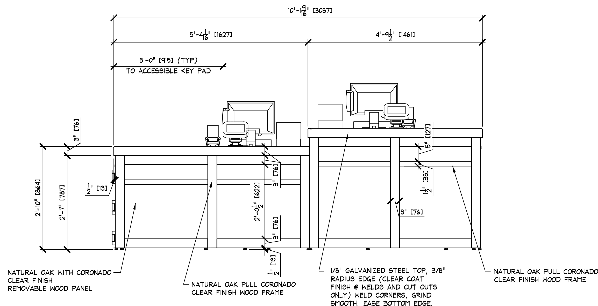
EXTERIOR ELEVATION
