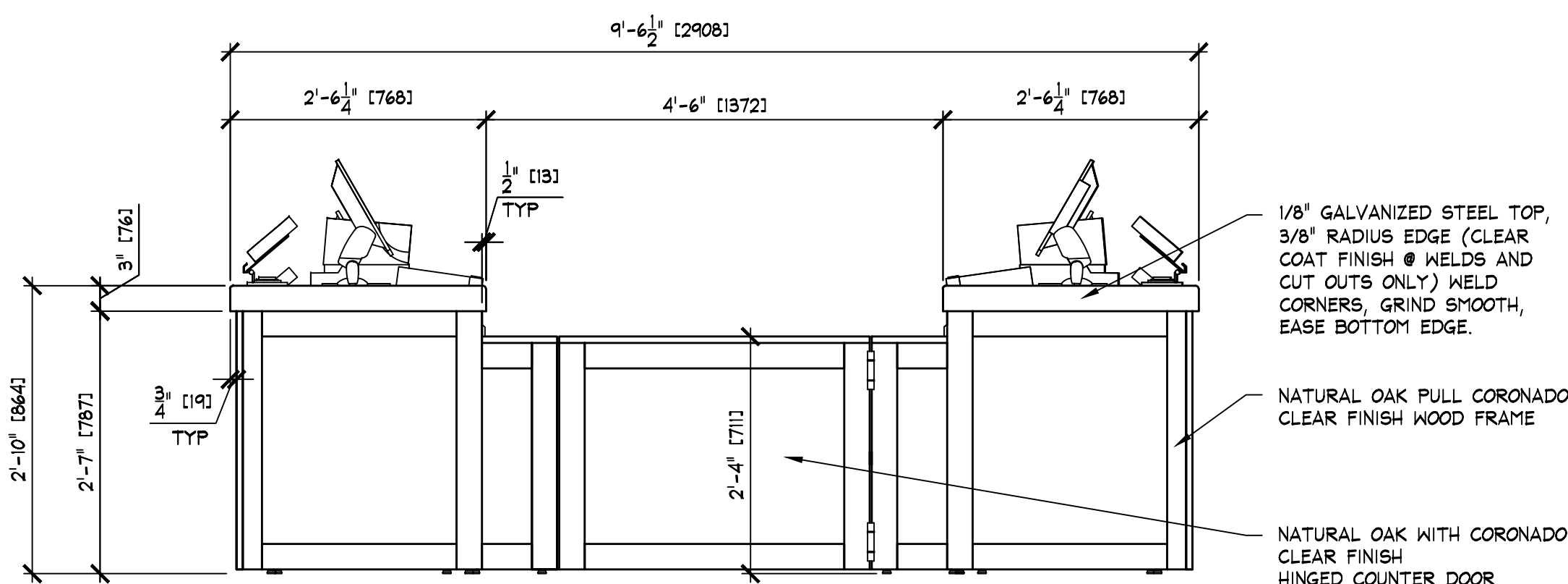
EXTERIOR ELEVATION
