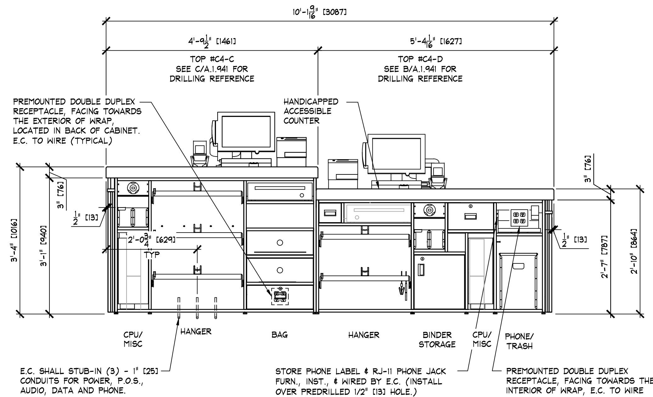
INTERIOR ELEVATION
