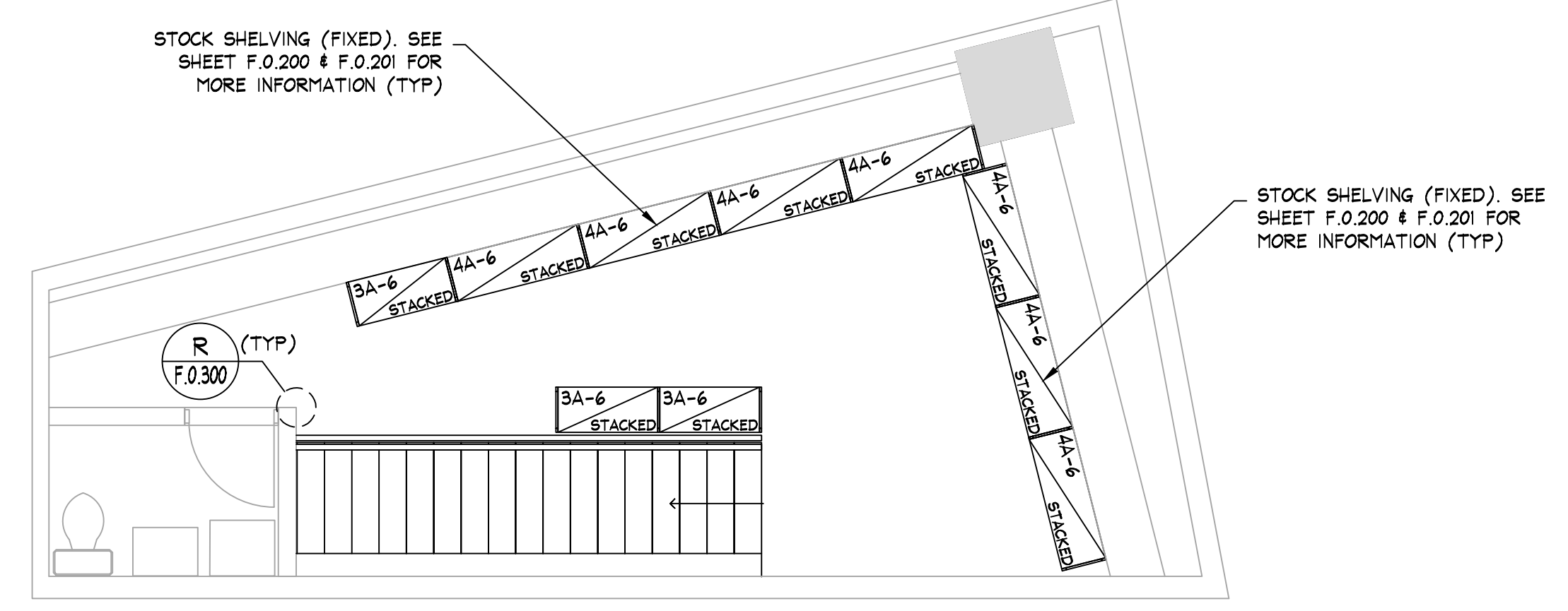
FIXTURE PLAN MEZZANINE SCALE: 1/4" = 1'-0" (1:50)
