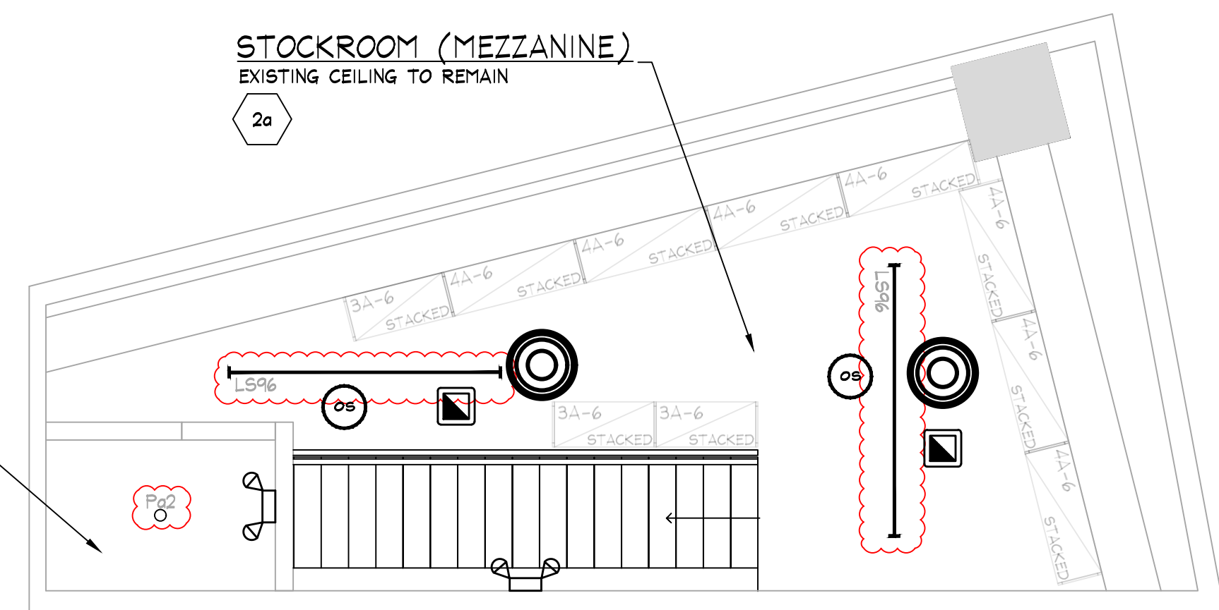
DEVICE COORDINATION REFLECTED CEILING PLAN MEZZANINE
