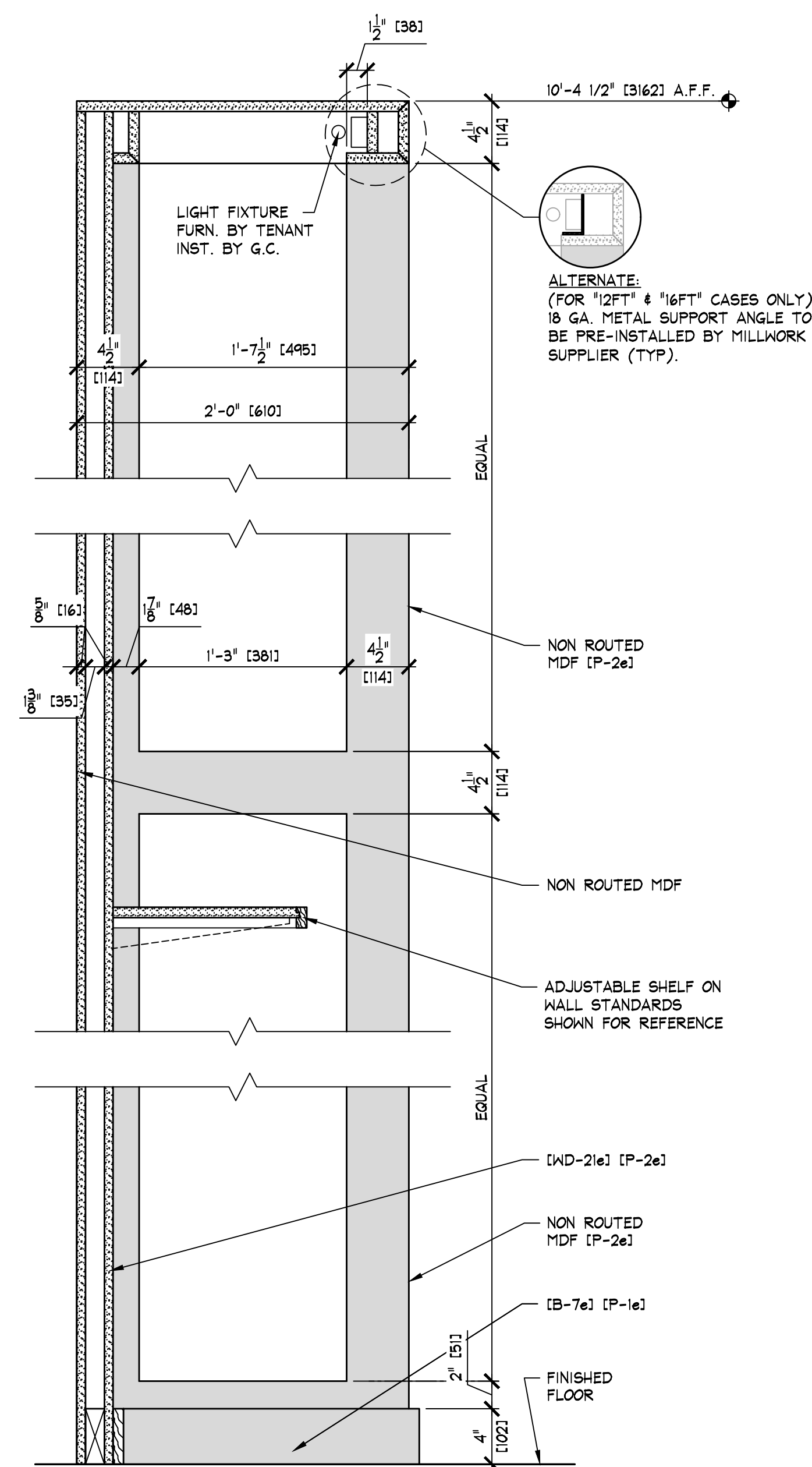
PREFAB. DISPLAY CASE ASSEMBLY 'D' SECTION SCALE: 1 1/2" = 1'-0" [1:8]
