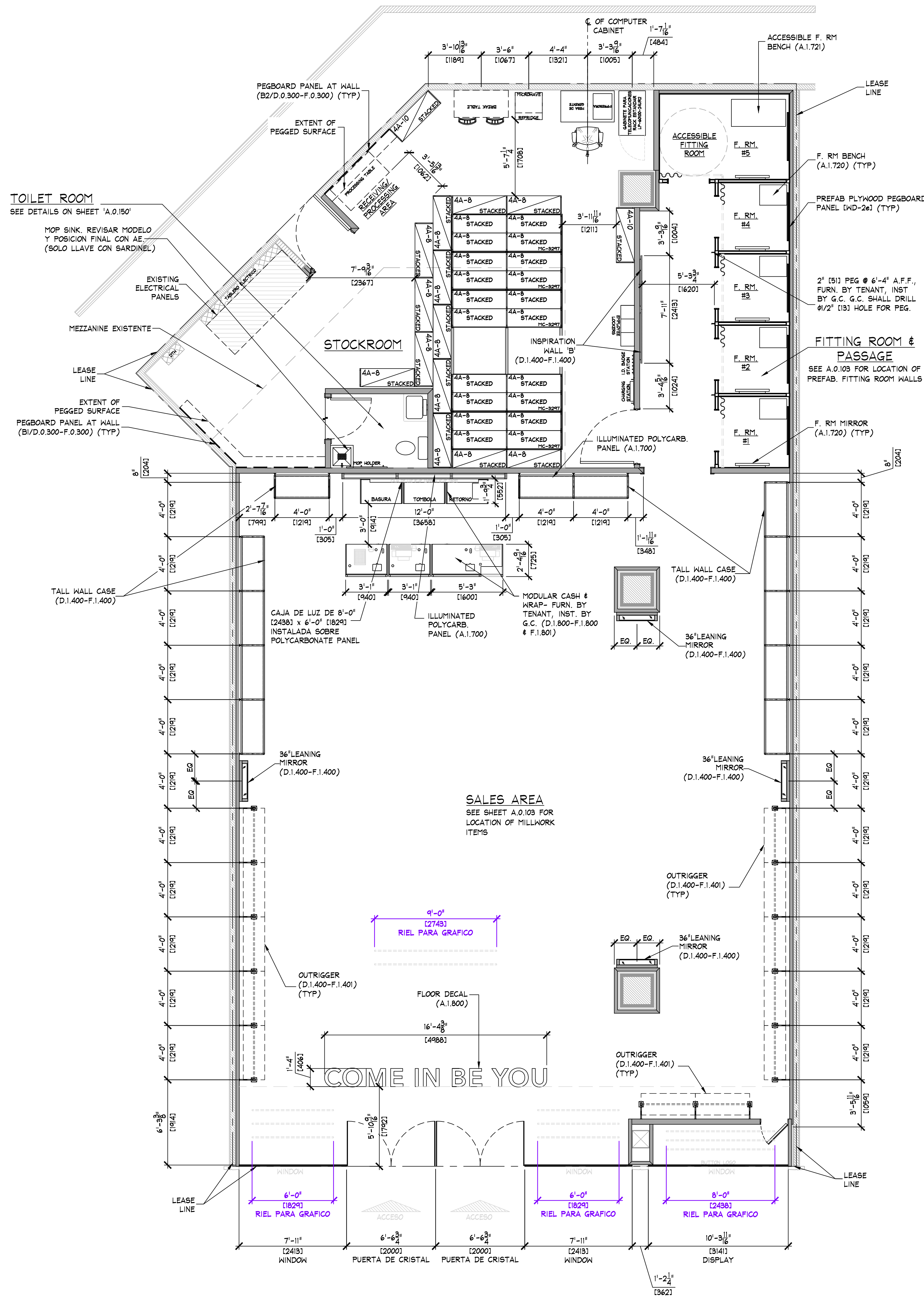
FIXTURE PLAN SCALE: 1/4" = 1'-0" (1:50)
