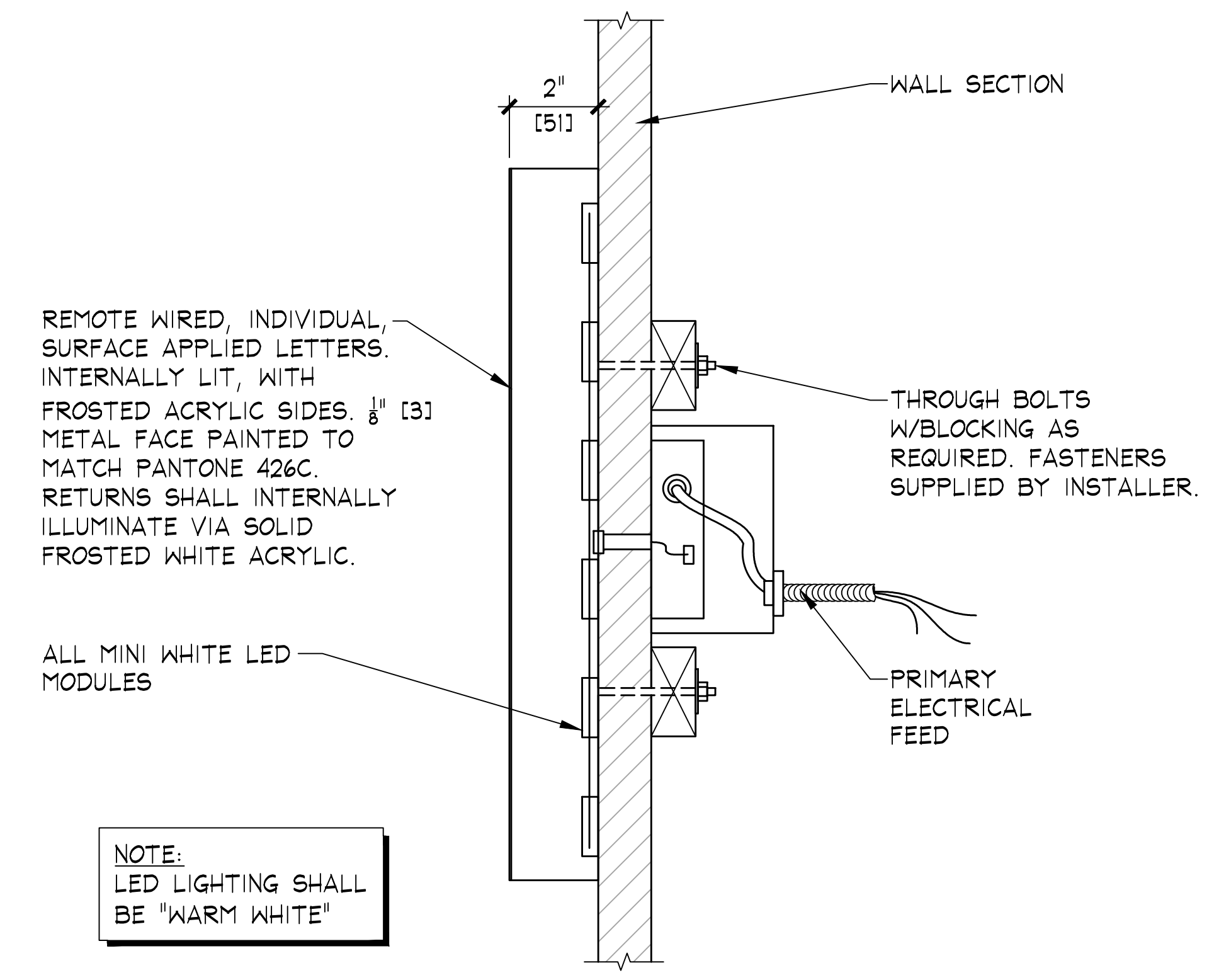
B SECTION VIEW A.1.800 SCALE: 3" = 1'-0" [1:4] (12-07-2017)
