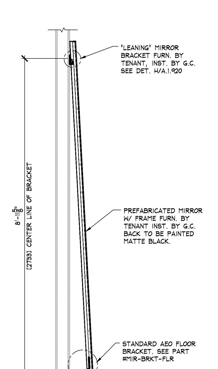
F "LEANING" MIRROR SECTION (LEANING) SCALE: 3/4" = 1'-0" [1:16]
