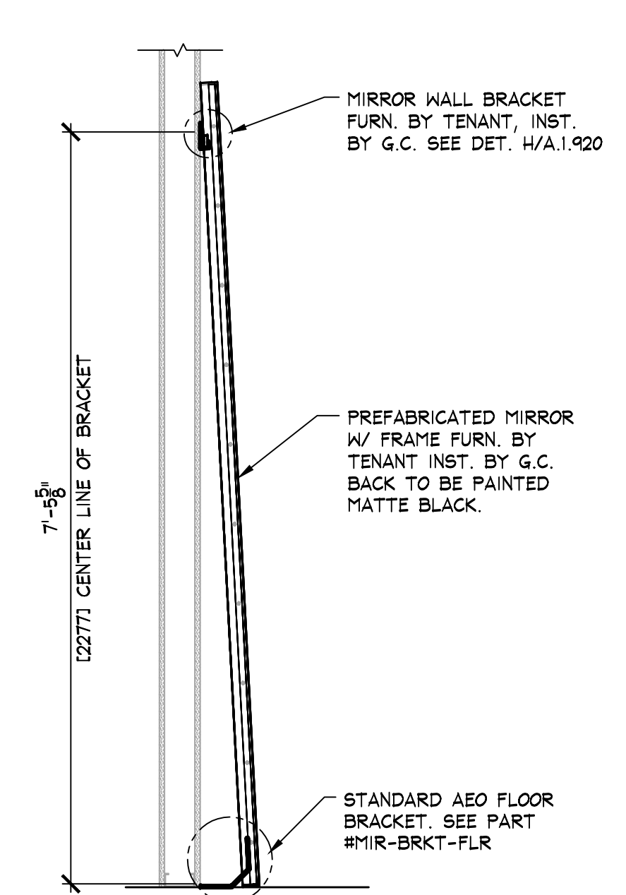
D "LEANING" MIRROR SECTION SCALE: 3/4" = 1'-0" [1:16]
