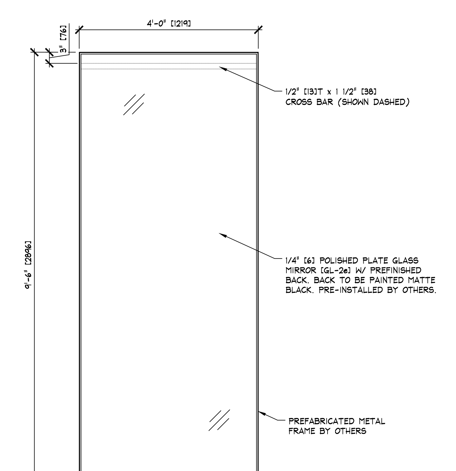
E SALES AREA MIRROR DETAIL SCALE: 3/4" = 1'-0" [1:16]
