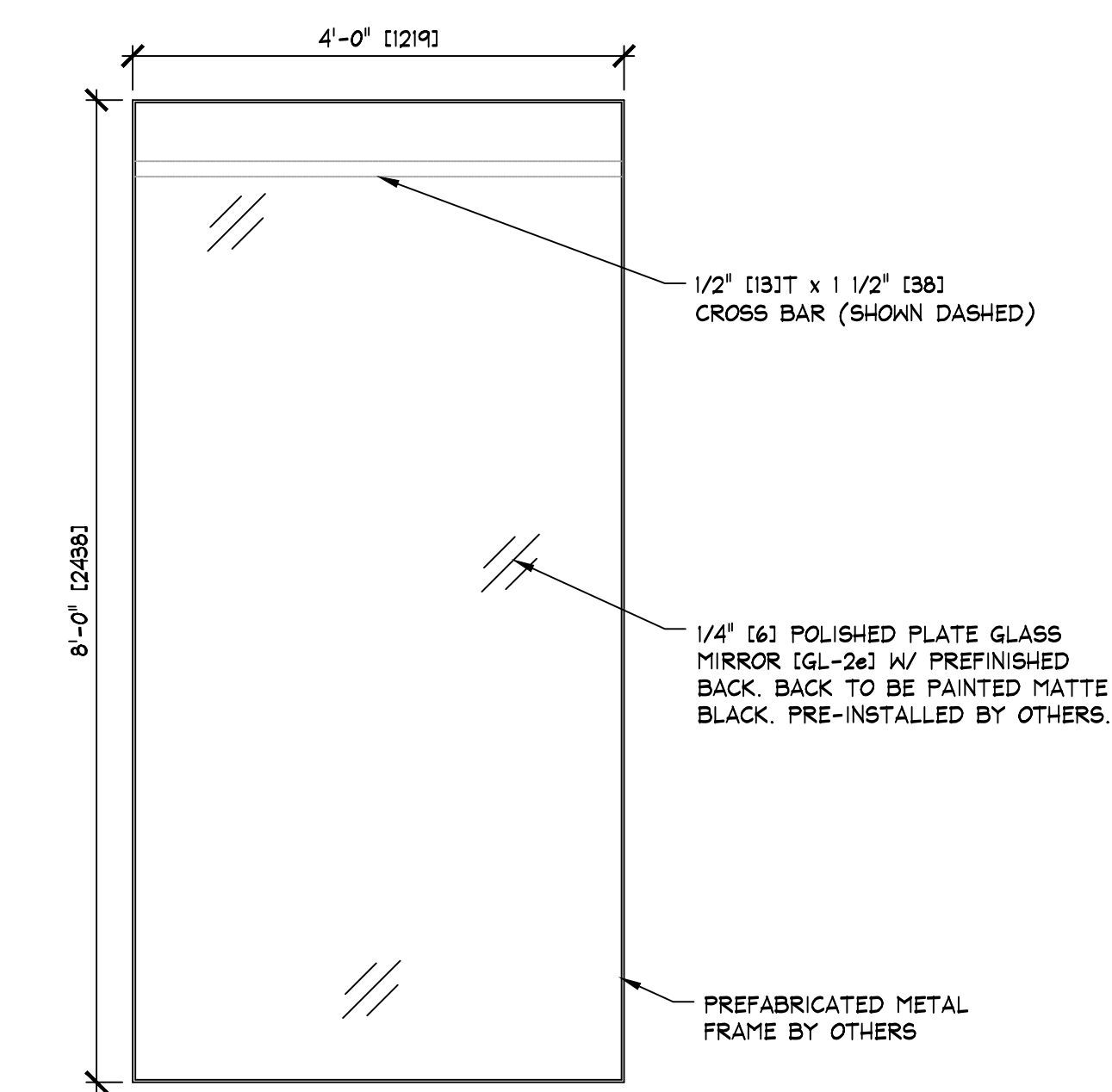
C PASSAGE MIRROR DETAIL SCALE: 3/4" = 1'-0" [1:16]
