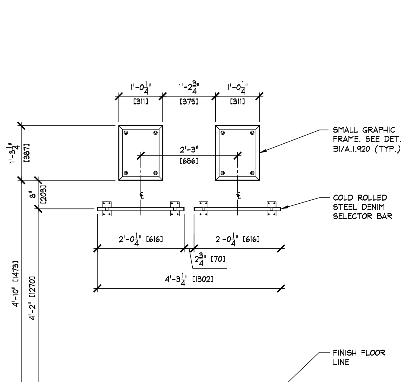
J GRAPHIC FRAME/DENIM BAR DETAIL SCALE: 3/4" = 1'-0" [1:16]
