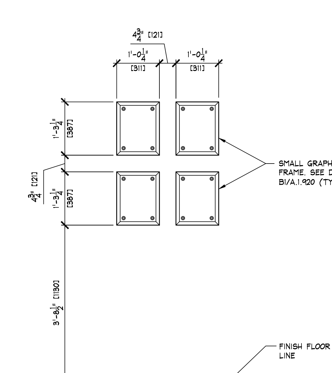
K GRAPHIC FRAME DETAIL SCALE: 3/4" = 1'-0" [1:16]
