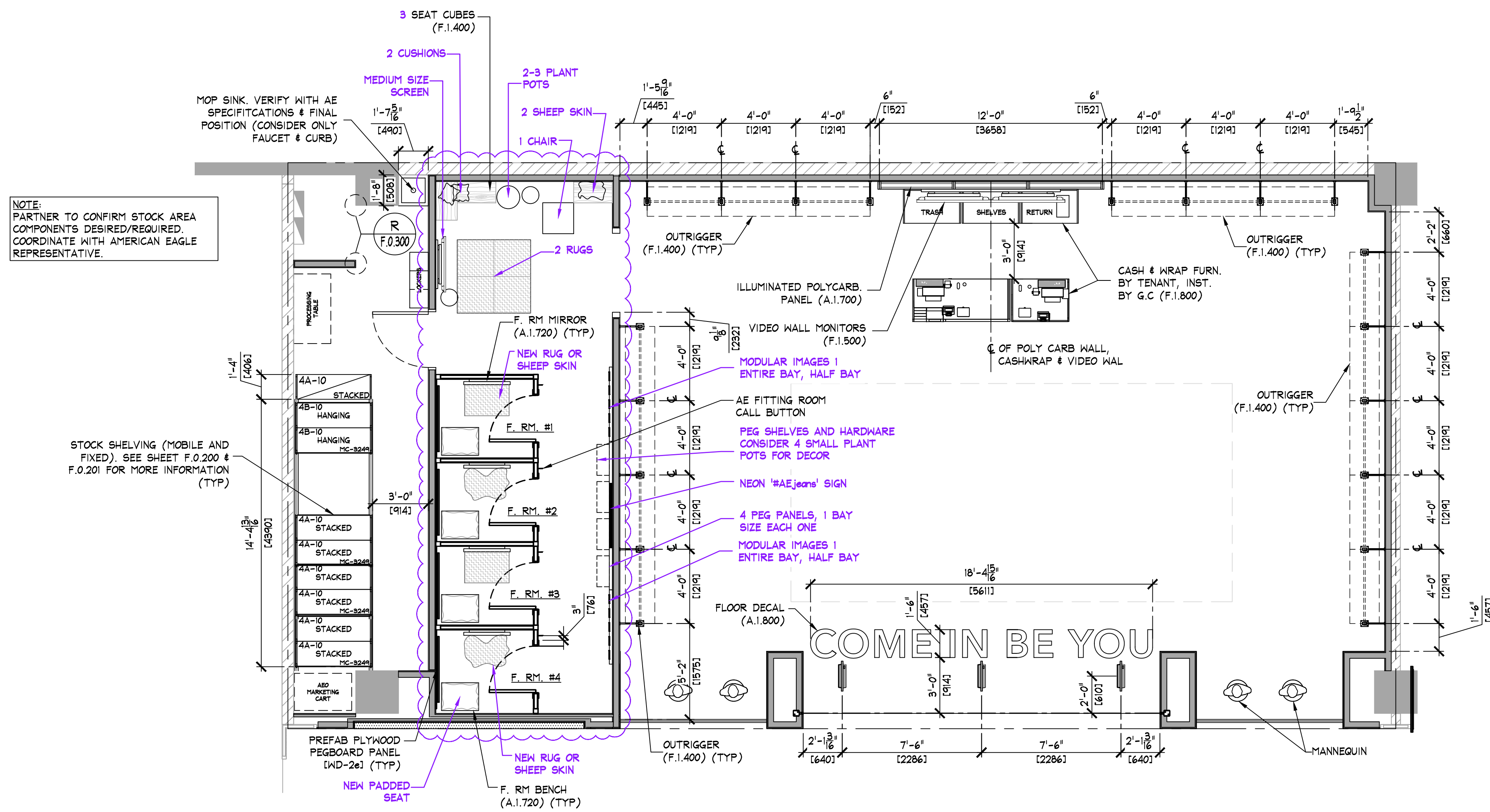
FIXTURE PLAN SCALE: 1/4" = 1'-0" (1:50)
