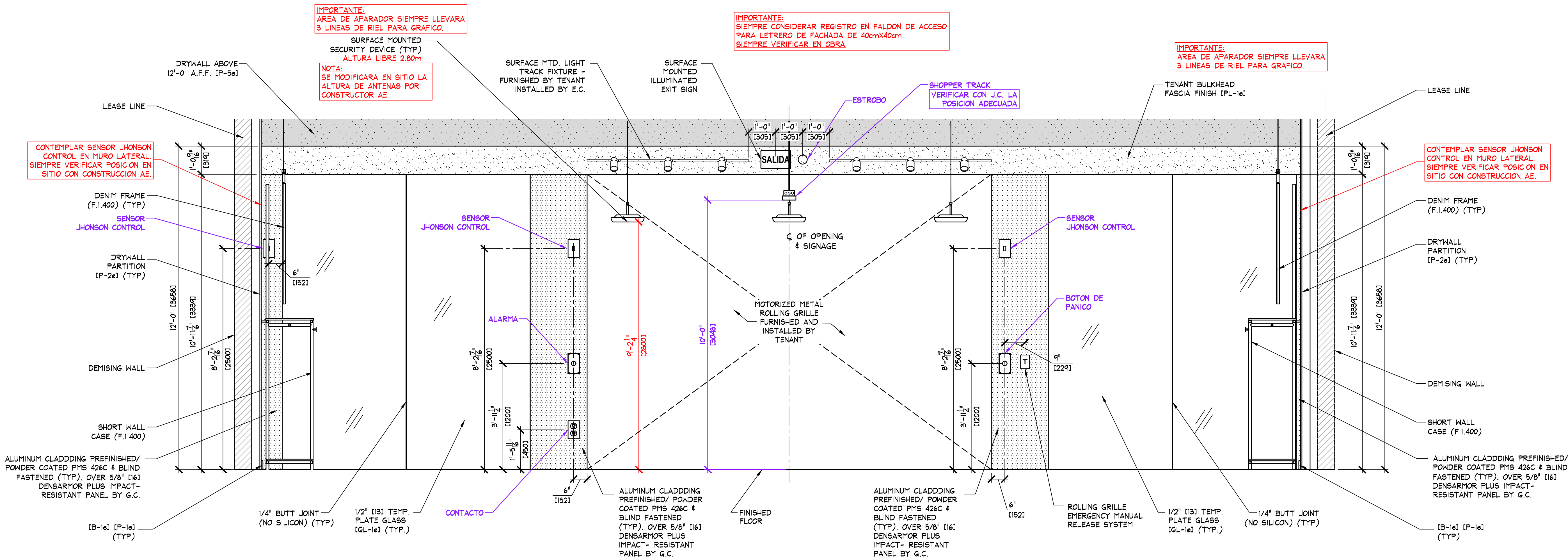
B INTERIOR ELEVATION SCALE: 1/2" = 1'-0" (1:25)
