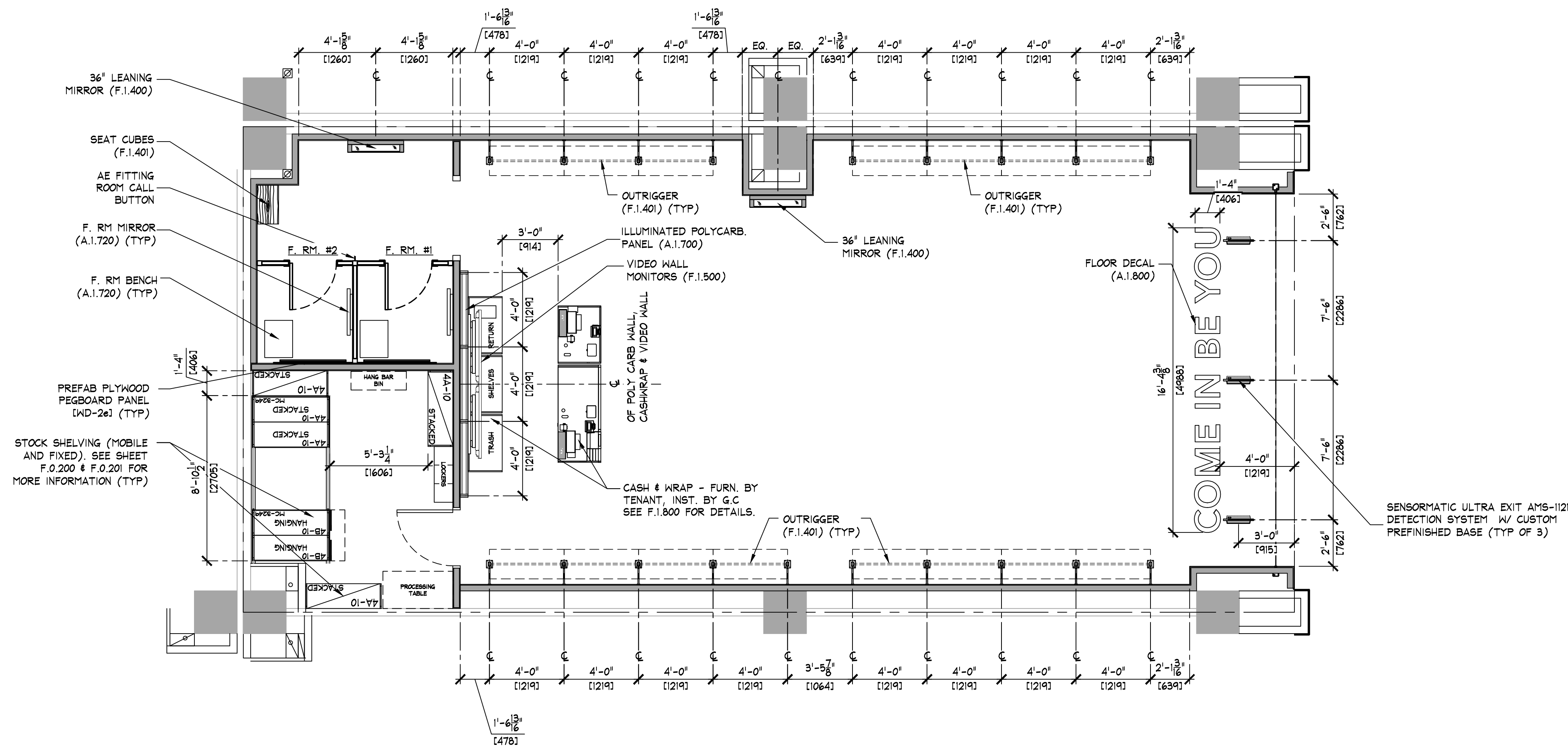
FIXTURE PLAN SCALE: 1/4" = 1'-0" (1:50)
