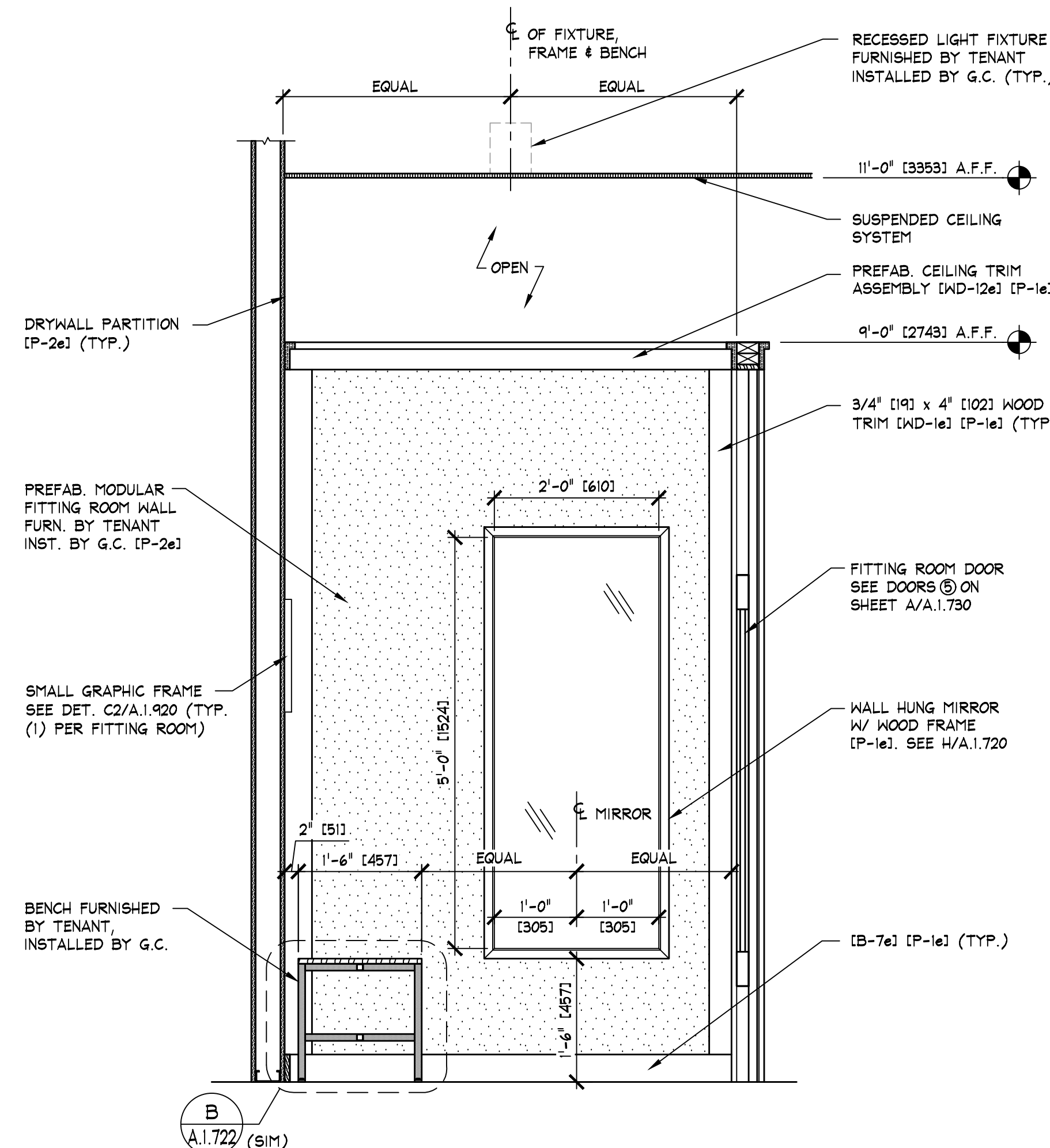
TYP. FITTING ROOM ELEVATION C.1.720 SCALE: 3/4" = 1'-0" [1:6]
