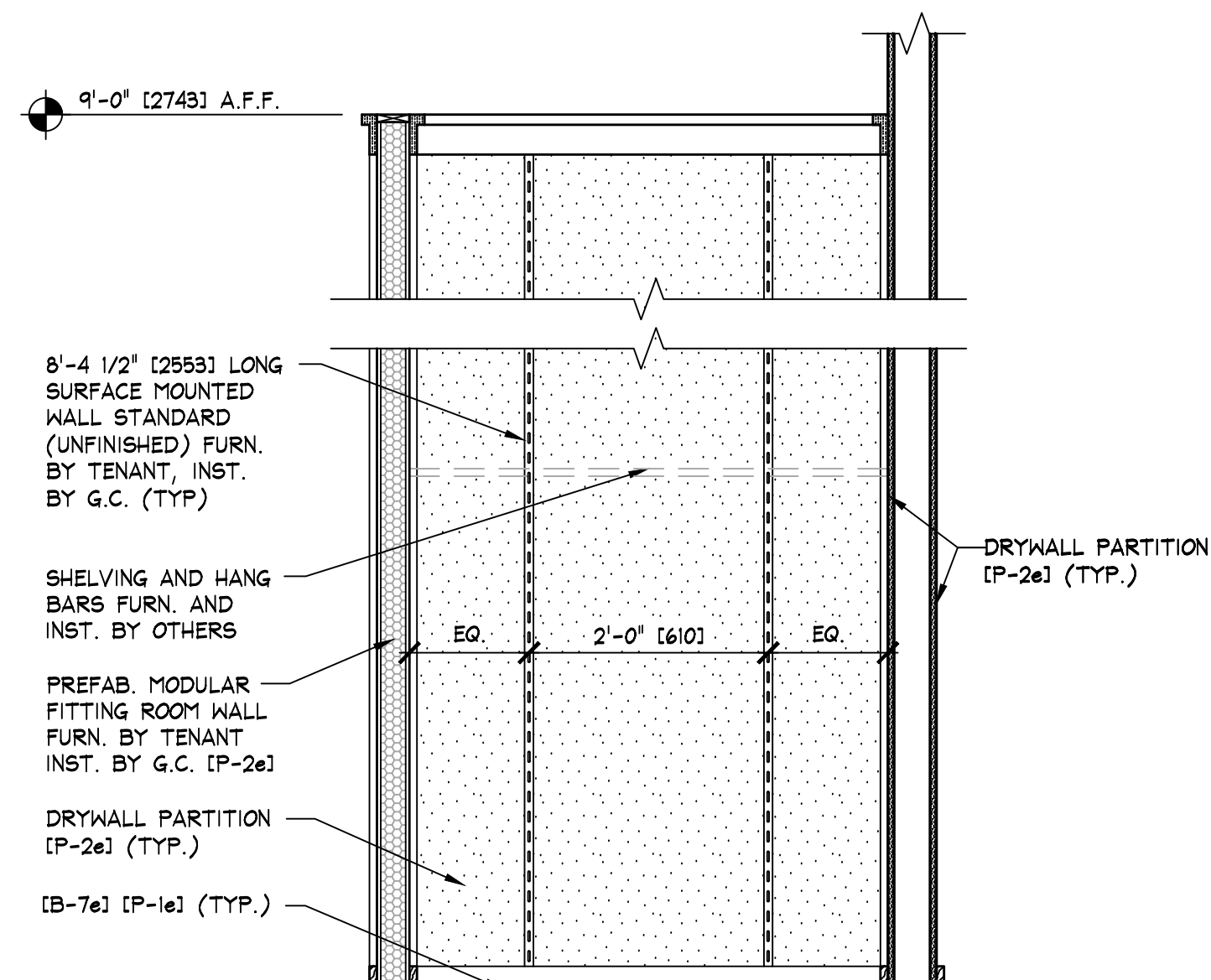
CLOSET DETAIL F2.1.720 SCALE: 3/4" = 1'-0" [1:6]
