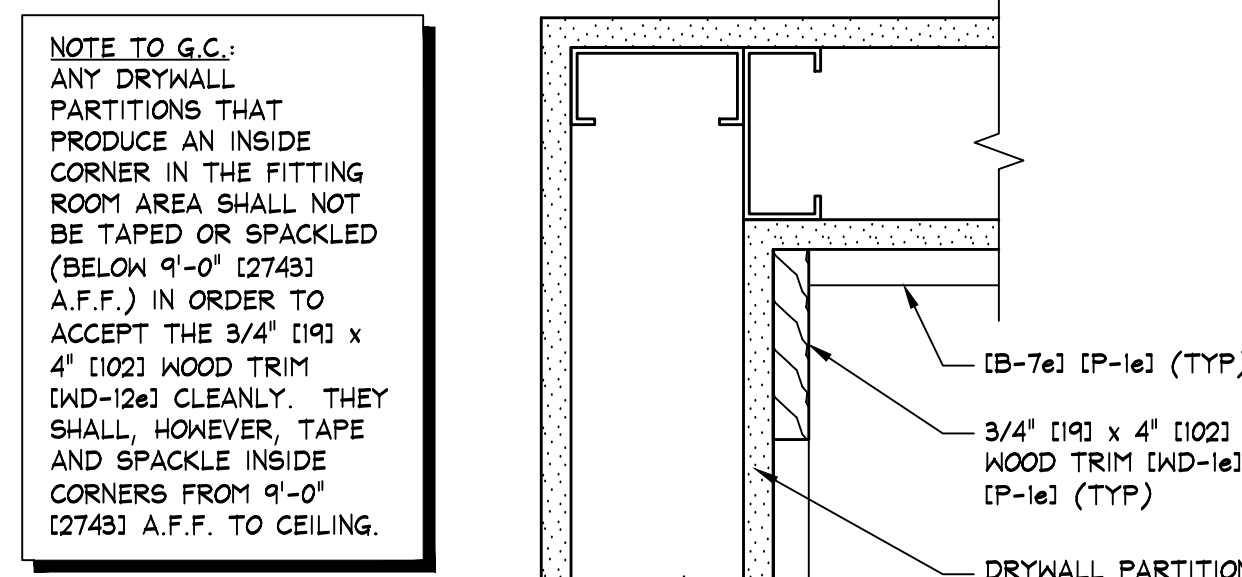
INSIDE CORNER DETAIL L.1.720 SCALE: 3" = 1'-0" [1:4]
