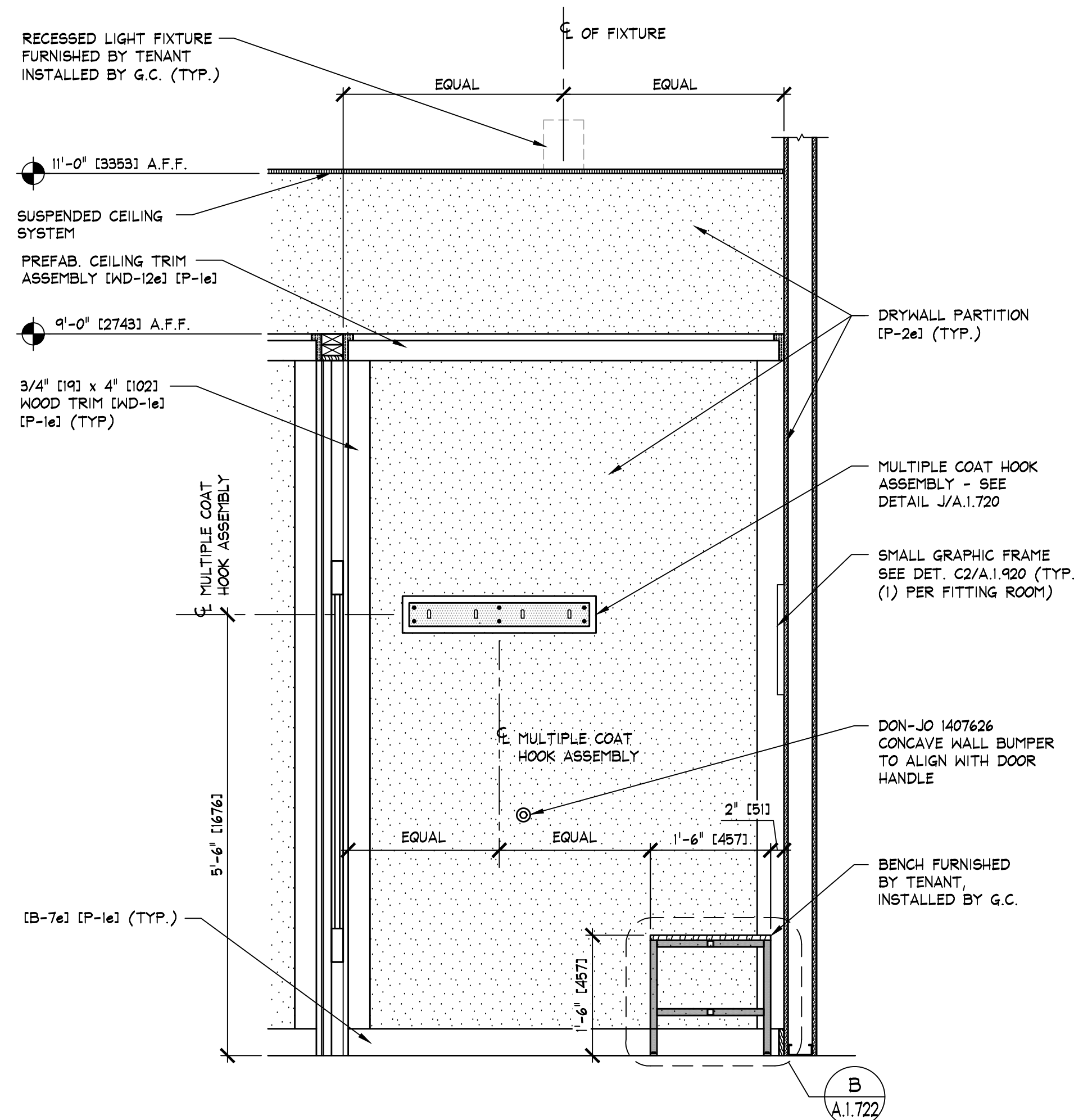
TYP. FITTING ROOM ELEVATION A.1.720 SCALE: 3/4" = 1'-0" [1:6]
