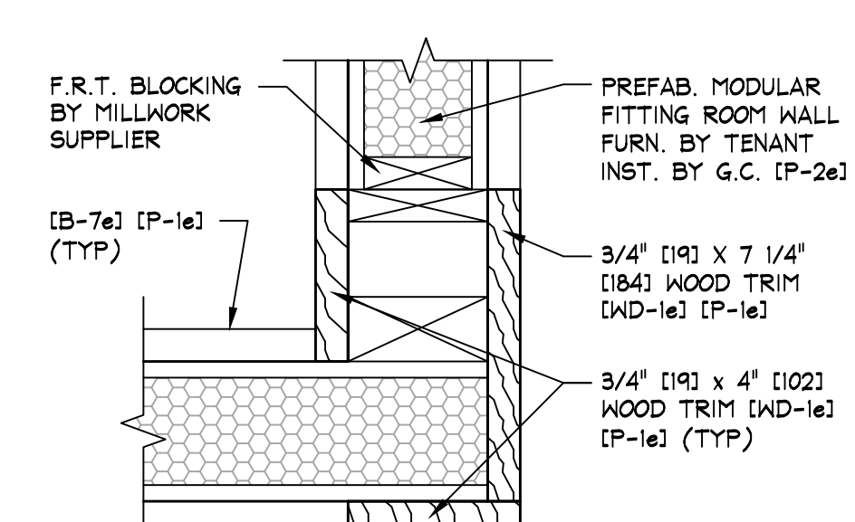
OUTSIDE CORNER TRIM DETAIL M.1.720 SCALE: 3" = 1'-0" [1:4]
