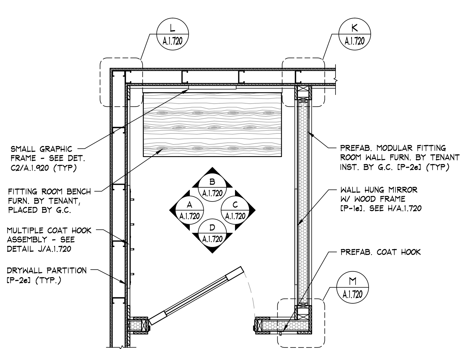
FITTING ROOM PLAN (TYP) E.1.720 SCALE: 3/4" = 1'-0" [1:6]
