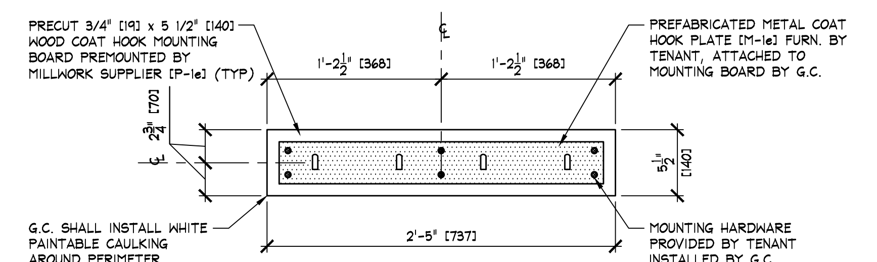
MULTIPLE COAT HOOK ASSEMBLY DETAIL J.1.720 SCALE: 1 1/2" = 1'-0" [1:8]
