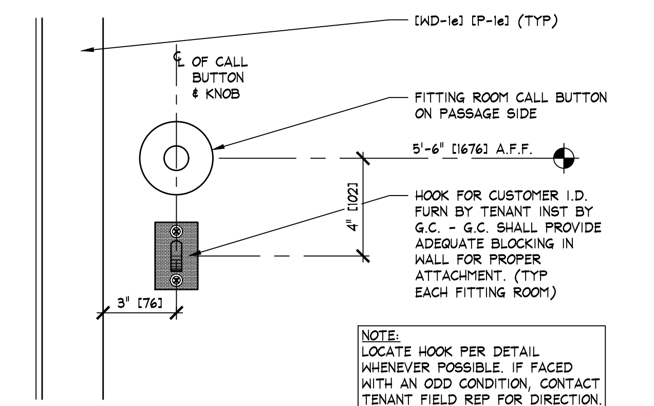
PASSAGE SIDE CALL BUTTON/HOOK DETAIL AA.1.720 SCALE: 3" = 1'-0" [1:4]
