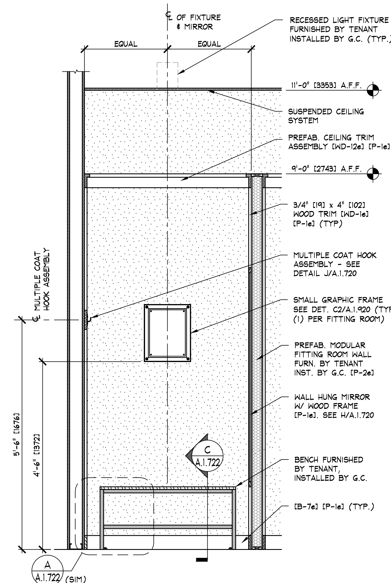
TYP. FITTING ROOM ELEVATION B.1.720 SCALE: 3/4" = 1'-0" [1:6]
