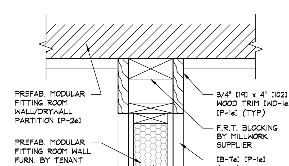
INSIDE CORNER DETAIL K.1.720 SCALE: 3" = 1'-0" [1:4]
