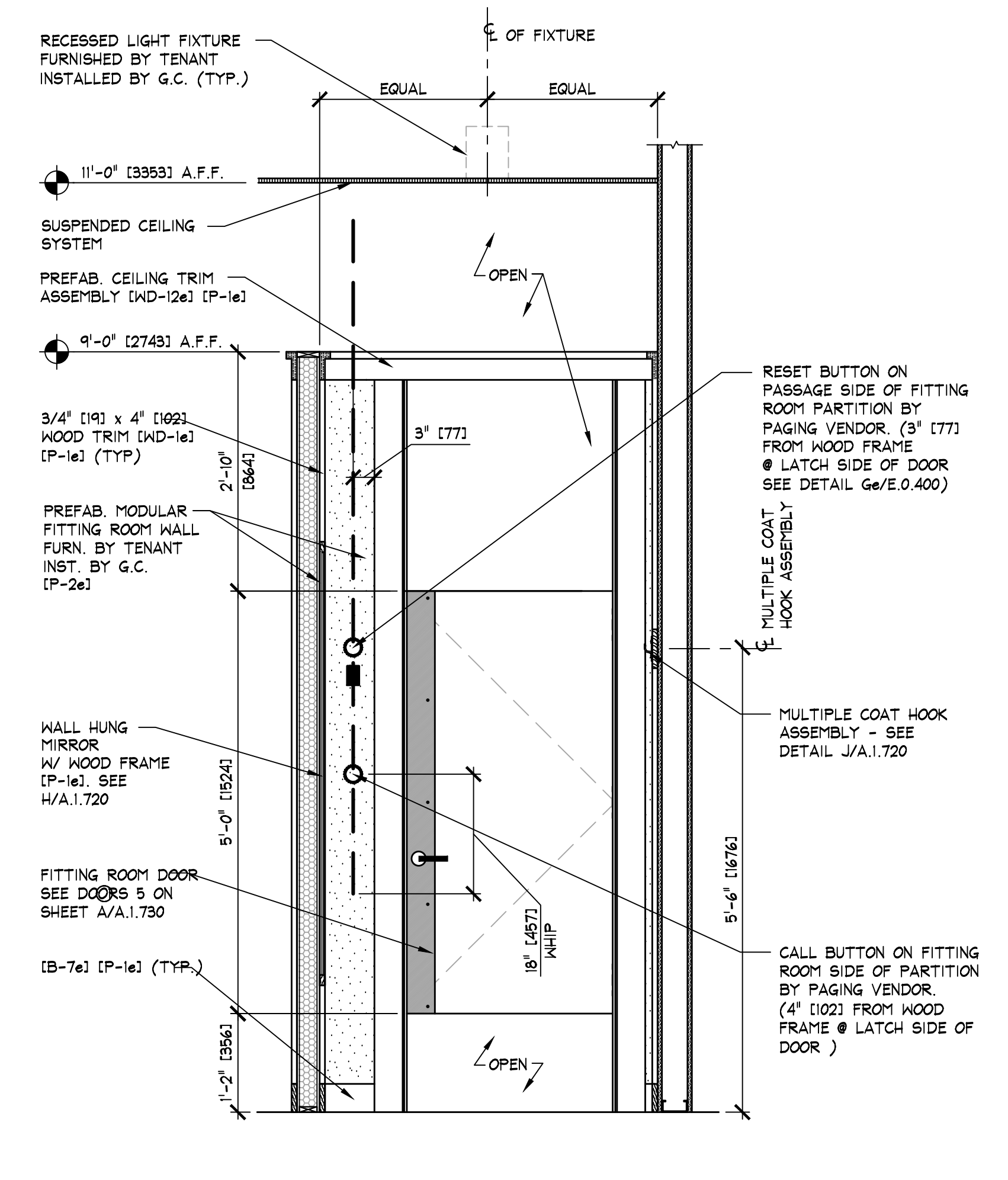
TYP. FITTING ROOM ELEVATION D.1.720 SCALE: 3/4" = 1'-0" [1:6]
