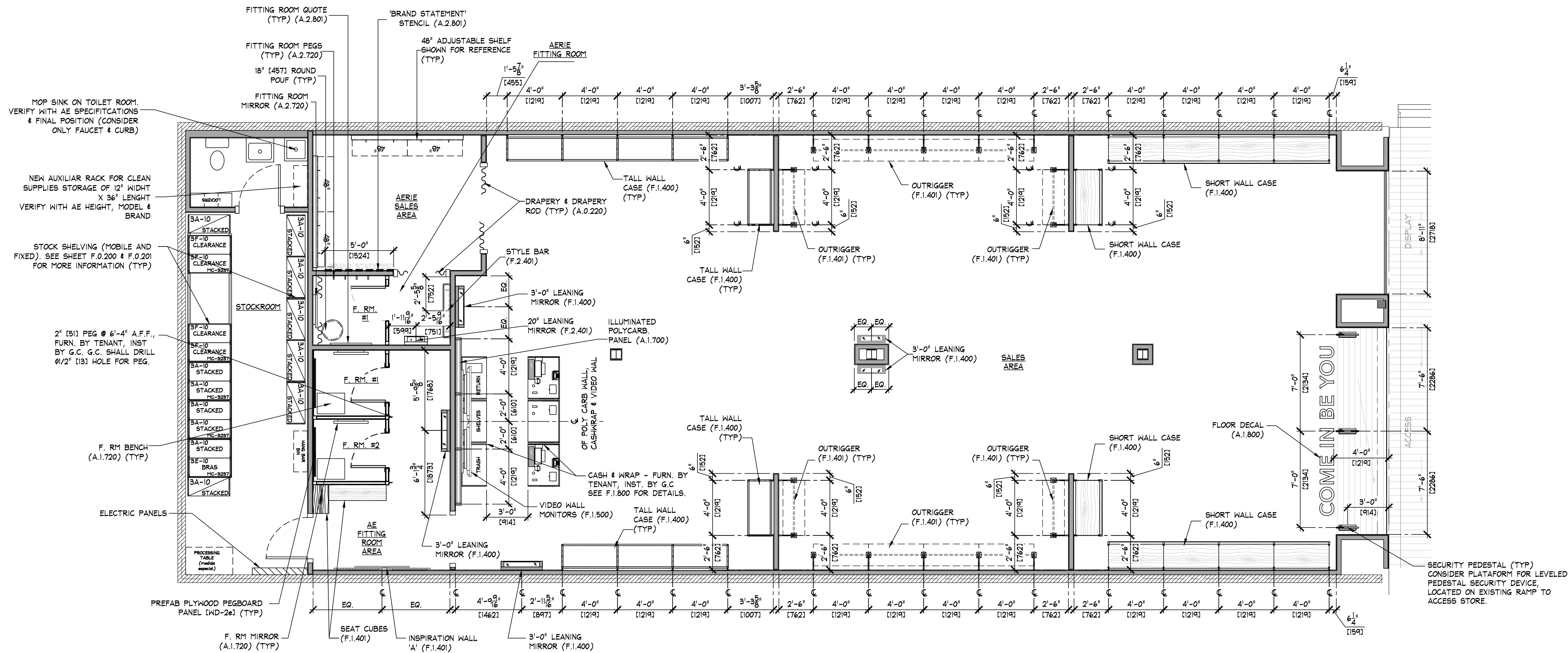
FIXTURE PLAN SCALE: 1/4" = 1'-0" (1:50)
