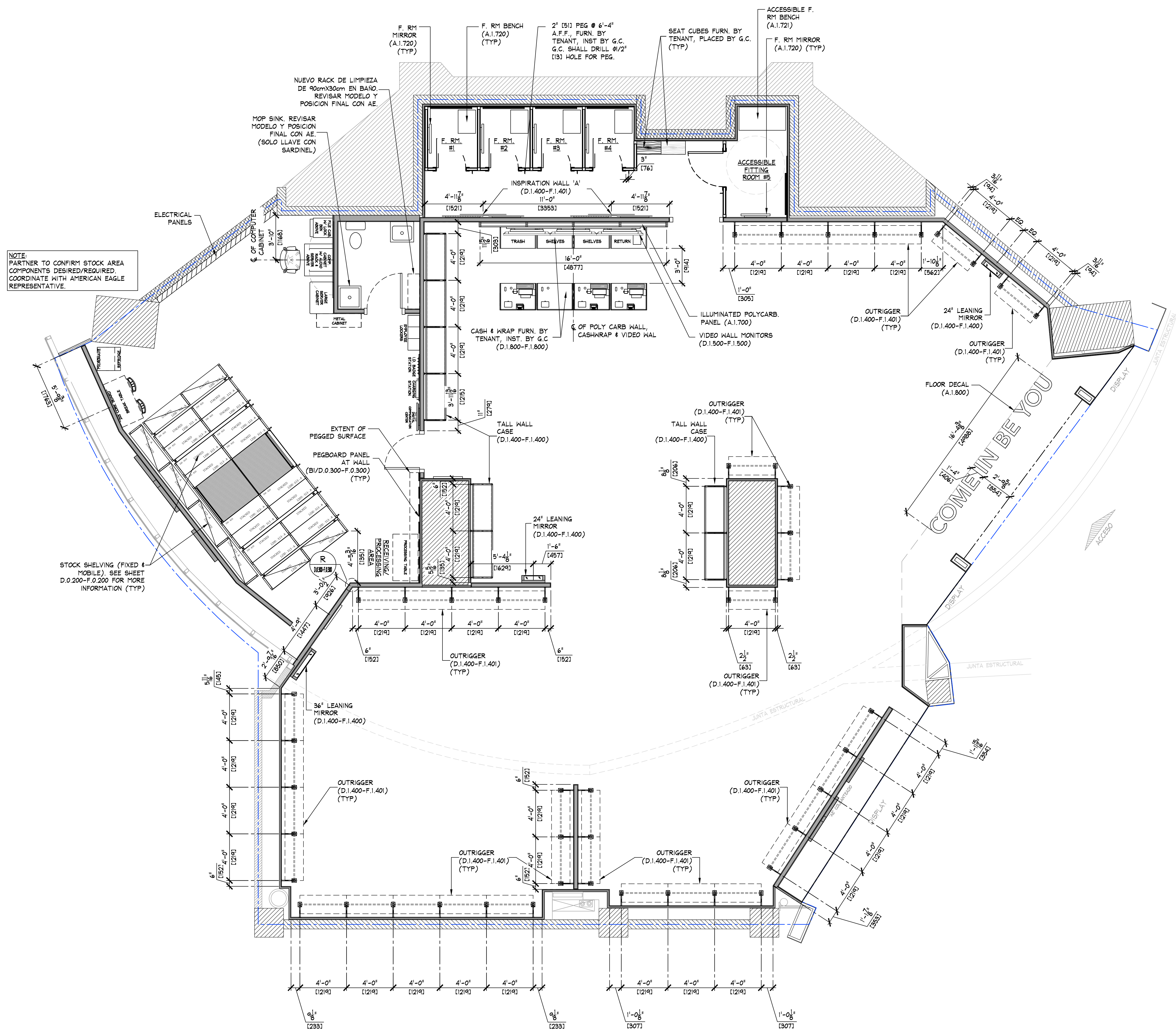
FIXTURE PLAN SCALE: 1/4" = 1'-0" (1:50)
