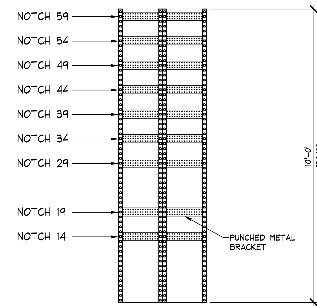
PREFAB PUNCHED METAL BRACKET MOUNTING DETAIL SCALE: 1/2"=1'-0" (FULL HEIGHT)
