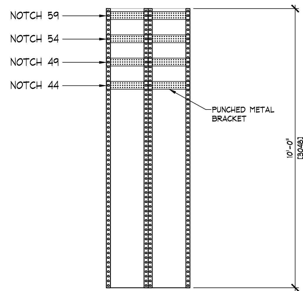
PREFAB PUNCHED METAL BRACKET MOUNTING DETAIL SCALE: 1/2"=1'-0" (PARTIAL HEIGHT)
