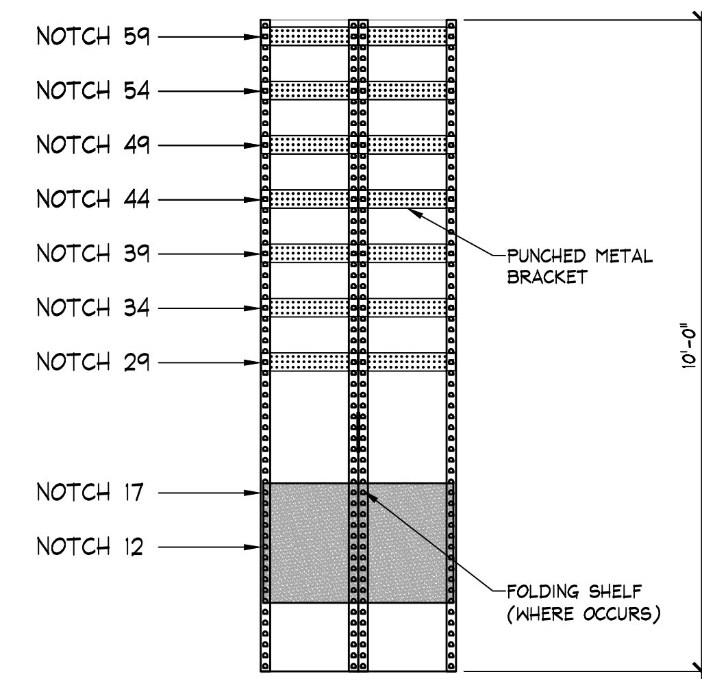
PREFAB PUNCHED METAL BRACKET MOUNTING DETAIL SCALE: 1/2"=1'-0" (W/ FOLDING SHELF)
